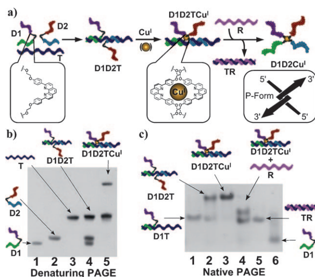
Figure 1. Templated synthesis of a DNA–metal junction with four different single-stranded arms. a) The template strand, T , hybridizes with D1 and D2 . \text{Cu}^{\text{I}} coordination links D1 and D2 , and then T can be removed by its complementary strand R to generate the single-stranded junction D1D2Cu I . b) Denaturing PAGE (12%, 4 M urea) analysis of \text{Cu}^{\text{I}} coordination to the hybridized structure: D1 (lane 1) and D2 (lane 2) on template T (lane 3). D1D2T completely denatured (lane 4); however, its \text{Cu}^{\text{I}} complex denatured to T and the metal-connected structure D1D2Cu I . c) Native PAGE (12%) analysis of the hybridization of D1 and D2 with template T (lane 2), \text{Cu}^{\text{I}} complexation (lane 3), and the displacement of T with its complementary strand R to generate TR and the fully single stranded junction D1D2Cu I (lane 4).
